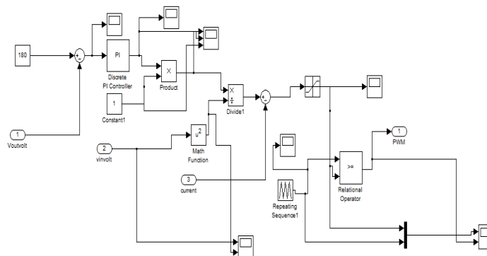
Fig.7. PWM Controller
