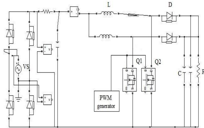
Fig. 5. Circuit diagram for the proposed system
