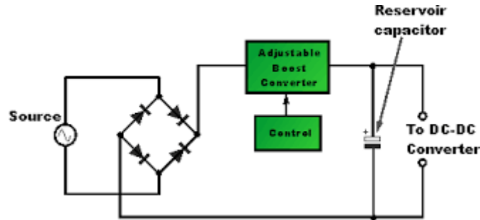
Fig. 3.A Typical PFC Circuit
