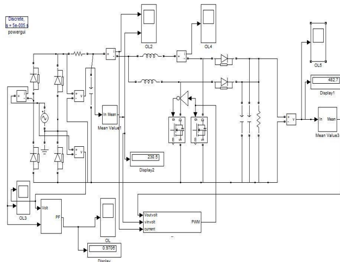
Fig. 6. Single stage high Power Factor Converter- Matlab circuit diagram.
