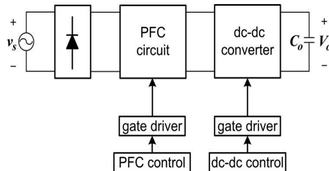
Fig.2.Two-Stage Single-Phase PFC Converter
