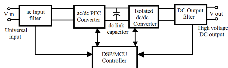
Fig. 1. Simplified system block diagram of a Universal battery charger.
