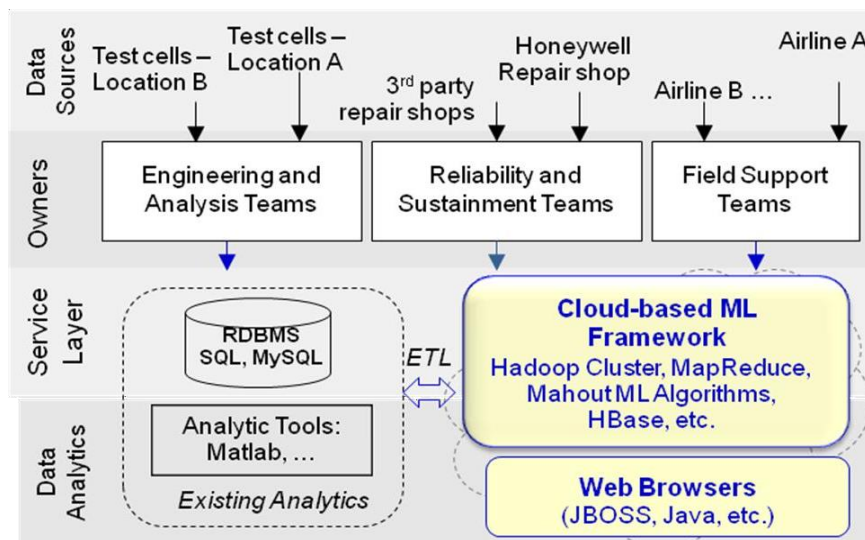
Figure 2: The Cloud-based ML Framework working with our existing data sources and analytic tools.
