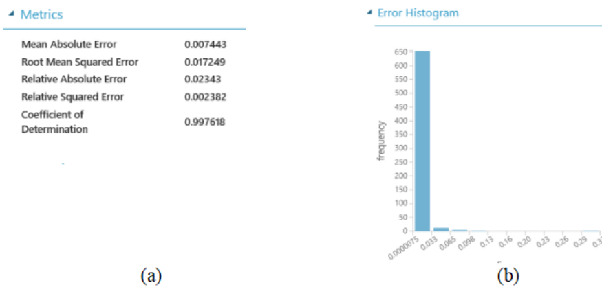
Figure7: Trained model evaluation of MTF prediction for PET imaging
