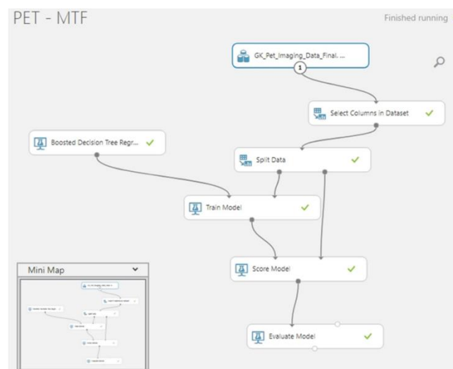
Figure6: ML workflow design
