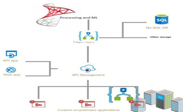
FIGURE 1: Serverless architecture
