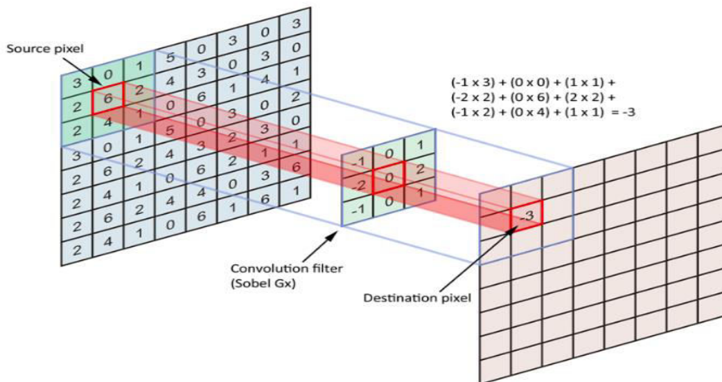
Fig. 3. The CNN Architecture filter
