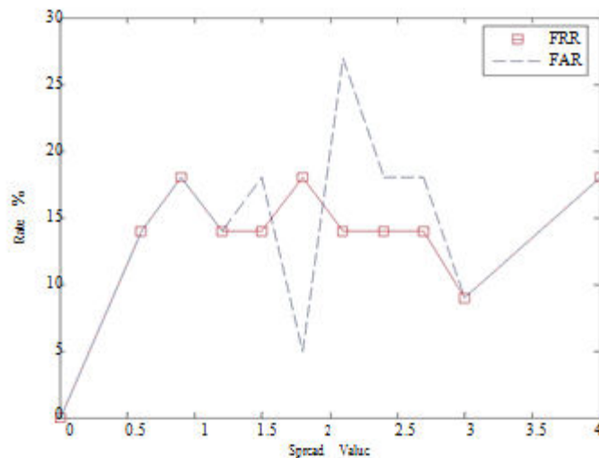
Figure 5. Spread vs. FAR and FRR (%)
