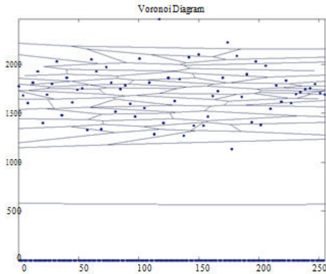
Figure 3. Voronoi diagram
