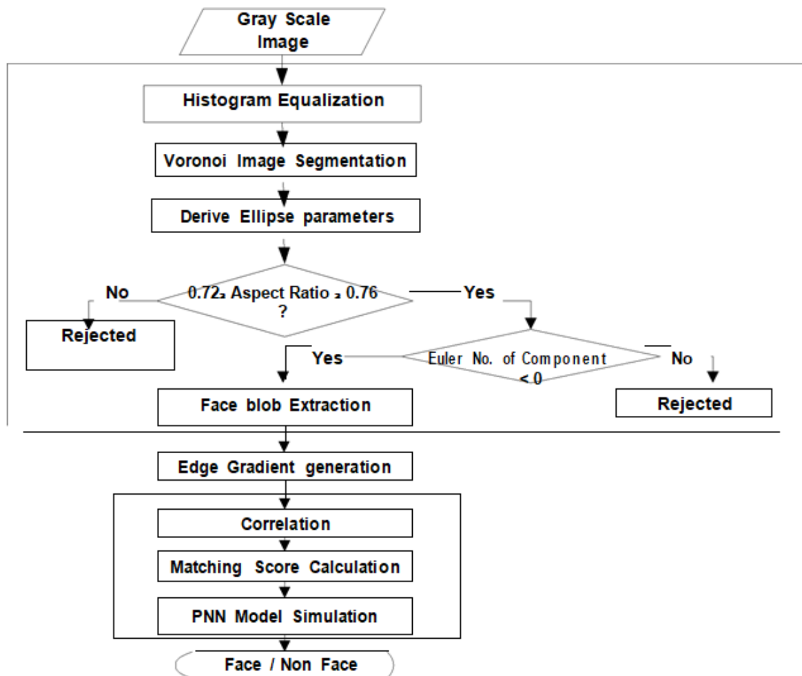
Figure 1. Schematic of face recognition diagram
