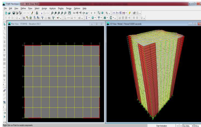
Fig 4.2.3 Time Period for Mode 3
