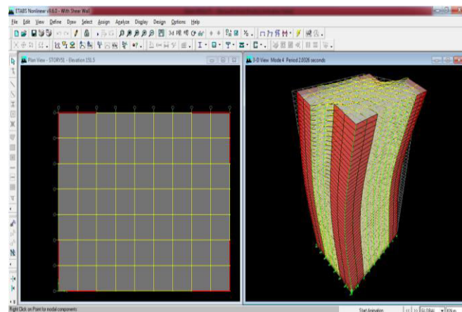
Fig 4.10 Time Period for Mode 4
