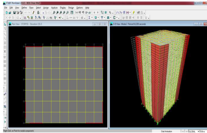
Fig 4.2.2 Time Period for Mode 2
