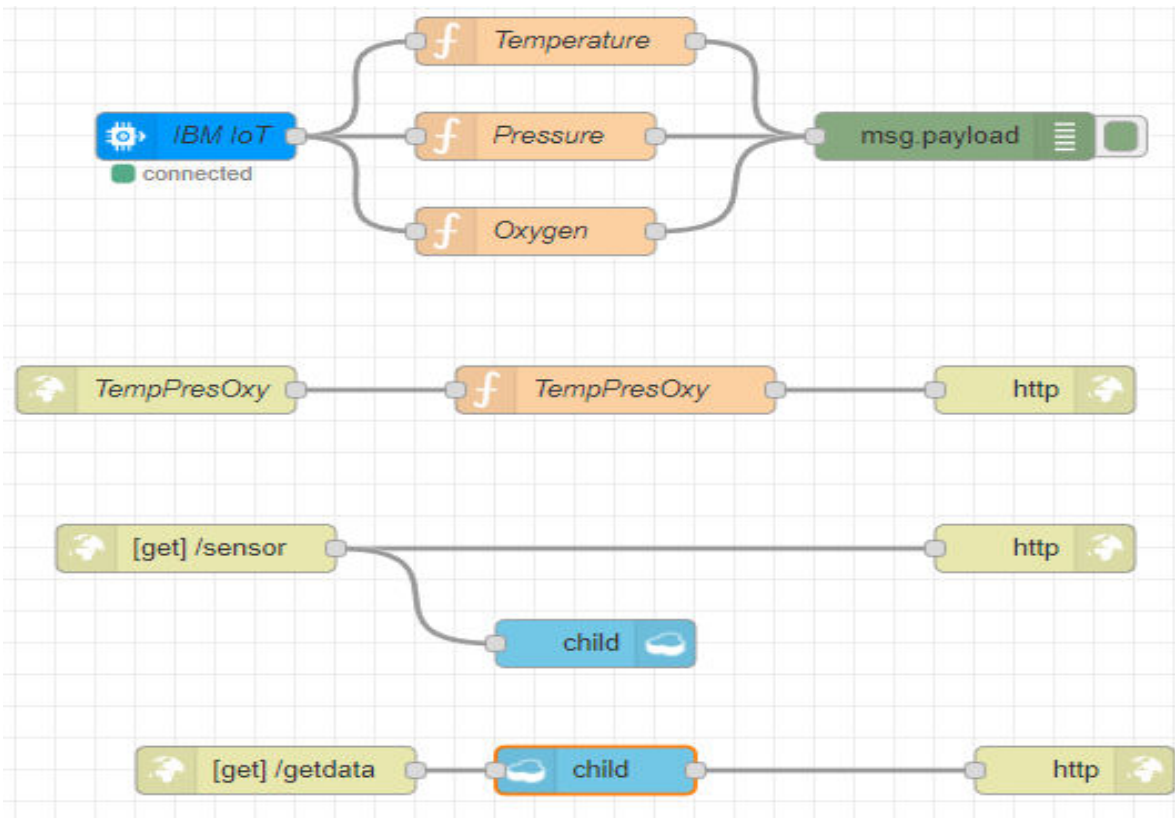
Fig 2.Simulation of sensors
