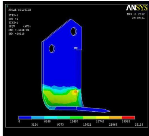
Analysis for 34mm radius Fig 12: High chromium steel
