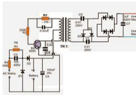
Fig.2. High voltage Low current circuit
