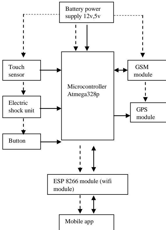
Fig. 1. BLOCK DIAGRAM OFIoT BASED SMART SECURITY AND SAFETY SYSTEM FOR WOMEN AND CHILDREN.
