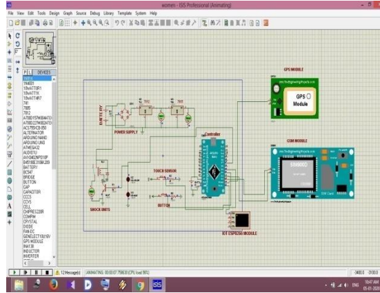
Fig.4. Simulation environment of the system.
