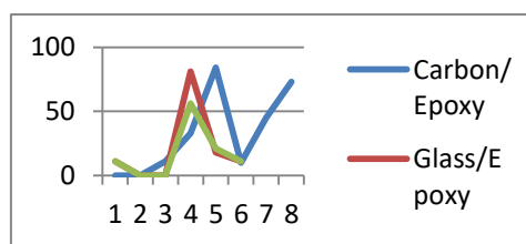
Graph (3.13): Maximum values of lamina stiffness components for different material among different lamina holds different fibre orientations.
