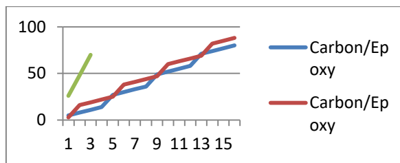
Graph (3.28): Minimum values of on axis longitudinal strain for carbon/epoxy among different planes
