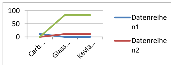
Graph (3.36): Minimum values of off-axis engineering elastic constants among different materials and different ply orientations.
