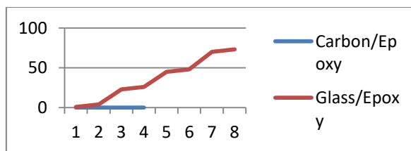
Graph (3.19): Maximum values of shear stress among different materials for different ply orientations.
