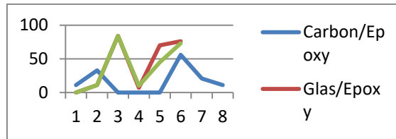
Graph (3.14): Minimum values of lamina stiffness components for different material among different laminas holds different fibre orientations.
