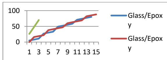
Graph (3.29): Maximum values of on axis longitudinal strain for glass/epoxy among different planes
