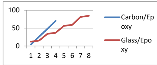
Graph (3.20): Minimum values of shear stress among different materials for different ply orientations.
