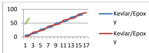
Graph (3.31): Maximum values of on axis longitudinal strain for Kevlar/epoxy among different planes
