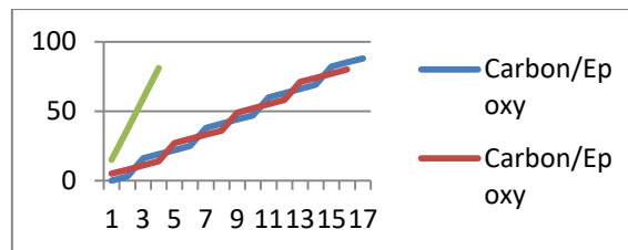
Graph (3.27): Maximum values of on axis longitudinal strain for carbon/epoxy among different planes
