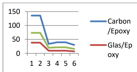
Graph (3.2): Maximum value comparison of laminar stiffness components as a function of changing orientation.
