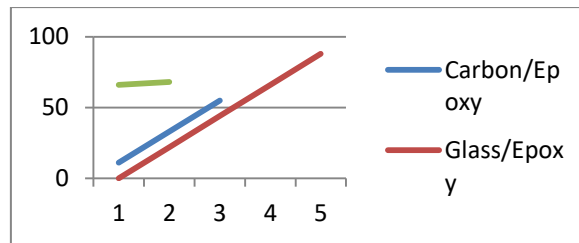
Graph (3.22): Minimum values of longitudinal off axis stress for different material among different ply orientations
