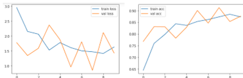
Fig 3: Result analysis of Leaf Disease Detection
