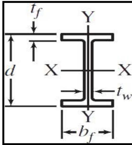
[Fig.4.1: Parallel flange section]
